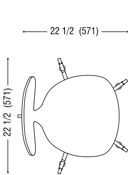
Plan View
