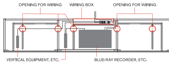
CROSS SECTION (TOP)
