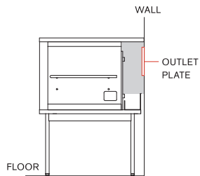
CROSS SECTION (SIDE)
