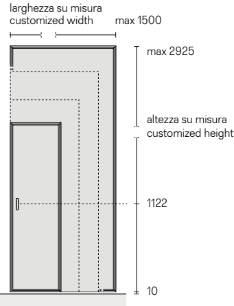
Dimensioni pannelli scorrevoli Sliding panel dimensions
