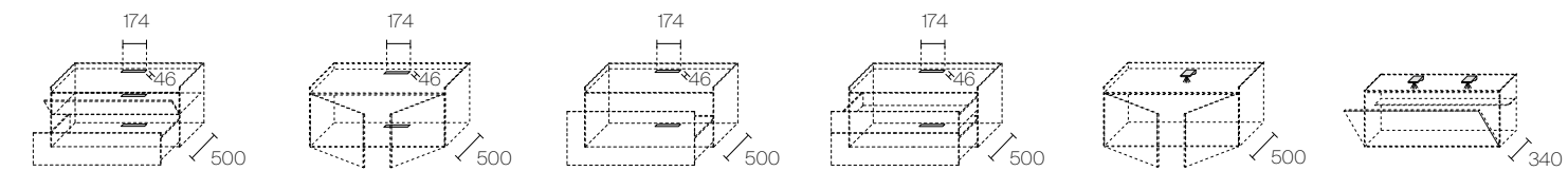
Optional cable duct for units depth 500. Not available for units with marble top.
