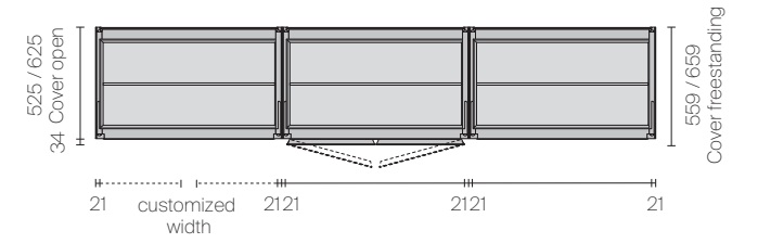
Linear composition Cover Open + Cover freestanding
