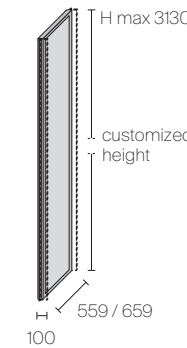
End panel (side passage opening)
