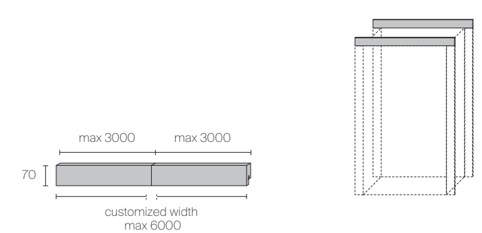
Double led lighting
