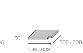
Corner floor base in lacquered wood or melamine
