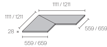
Corner top and floor base in lacquered wood or melamine
