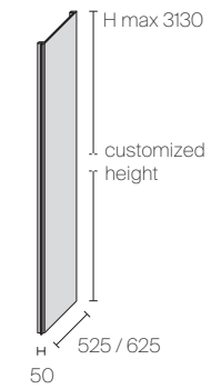
Side panel (middle room)
