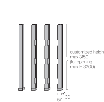
Structural upright
