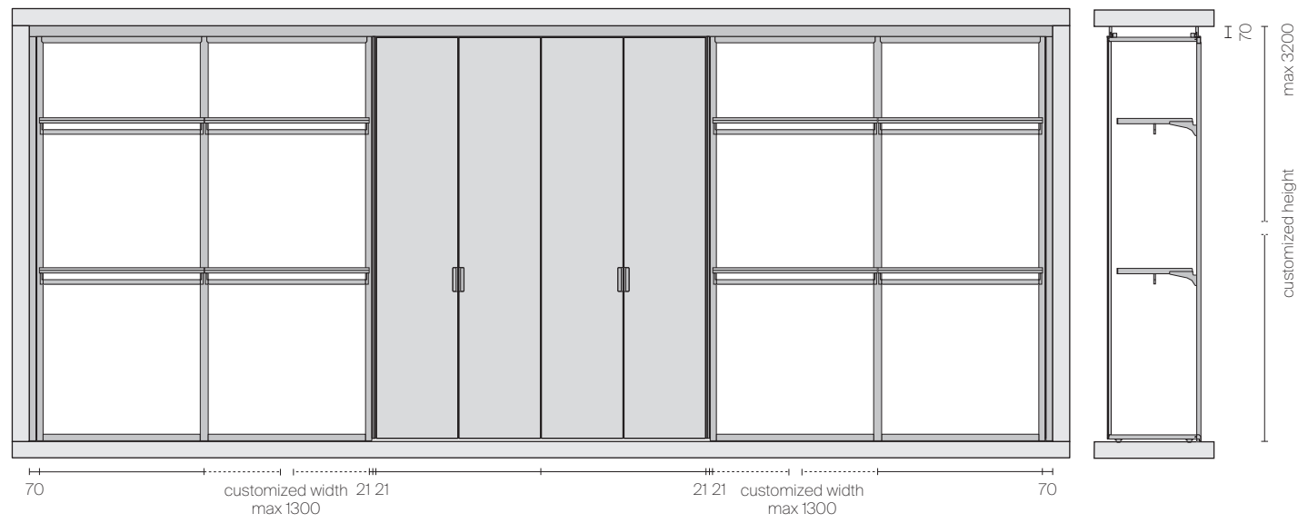
Cover Open + Cover freestanding
