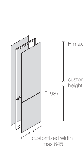
Double finished swing door with optional crosspieces
