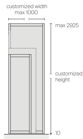
Folding and swing panel dimensions
