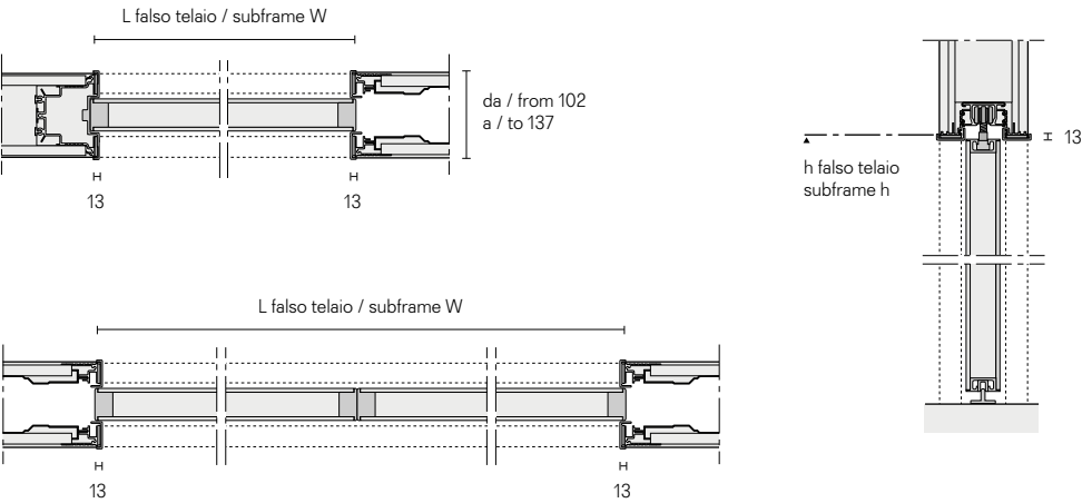
A. Luce netta falso telaio / Measure of the subframe C. Luce netta passaggio / Dimensions of the opening
